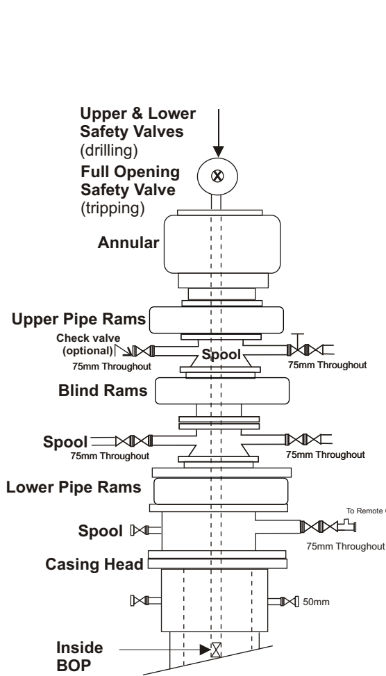
BLOWOUT PREVENTION STACK
