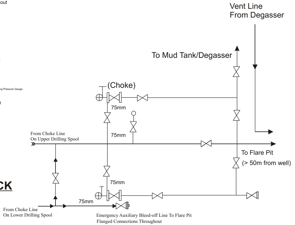
MANIFOLD SYSTEM
