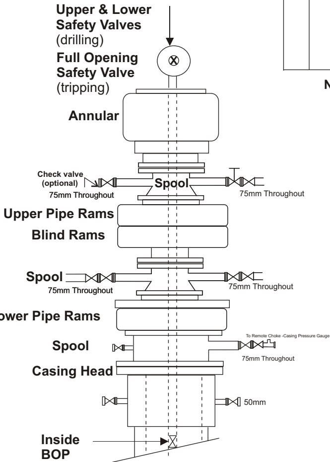
BLOWOUT PREVENTION STACK
