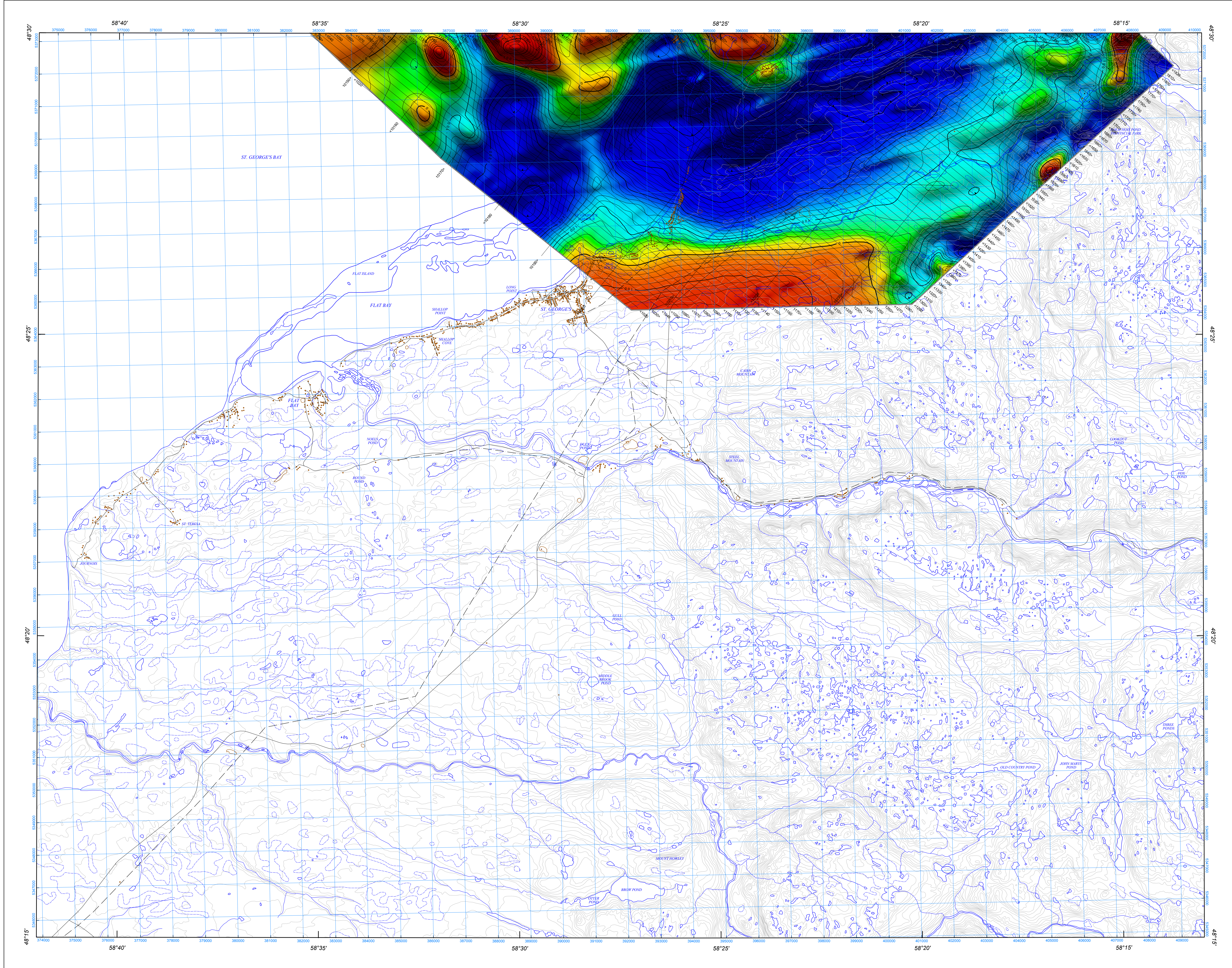
MAP 2009-55 FLAT BAY / MAIN GUT - NTS 12B/07 (east) & 12B/08 (west) Scale 1:50 000 kilomètres 1 0 1 2 3 4 5 kilomètres NAD83 / UTM zone 21N Digital Topographic Data provided by Geomatics Canada, Natural Resources Canada
