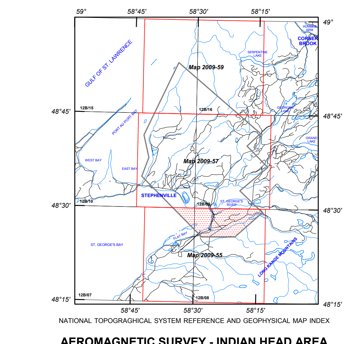
NATIONAL TOPOGRAPHICAL SYSTEM REFERENCE AND GEOPHYSICAL MAP INDEX AEROMAGNETIC SURVEY - INDIAN HEAD AREA
